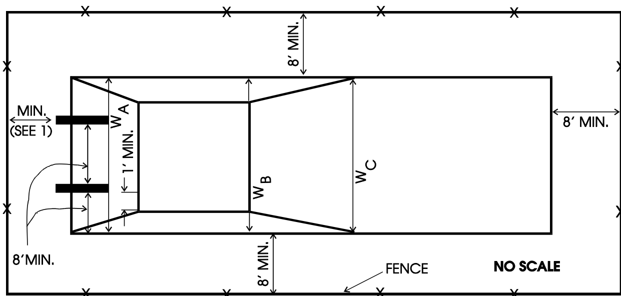
FIG. 2 POOL PLAN (RECTANGULAR) SHOWING MINIMUM DIMENSIONS. 1. 4 FEET MINIMUM FOR POOLS 3000 SQ. FT. OR LESS. 8 FEET MINIMUM FOR POOLS GREATER THAN 3000 SQ. FT.
