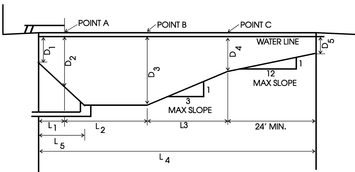
FIG. 1 POOL PROFILE SHOWING MINIMUM DIMENSIONS NO SCALE
